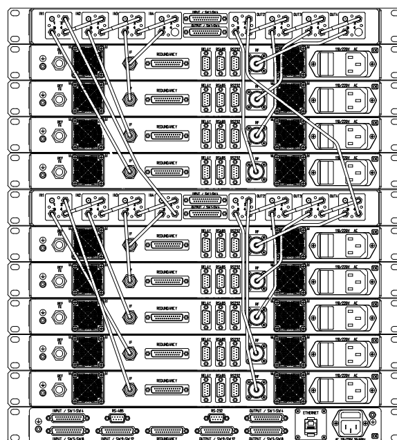
Rear View 1:8 Redundant System shown
