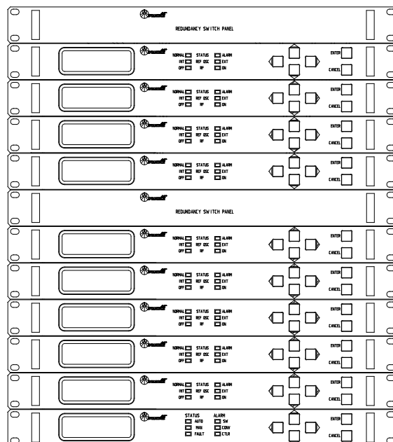
Front View of 1:8 Redundant System shown
